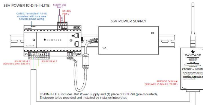
wiring diagram
